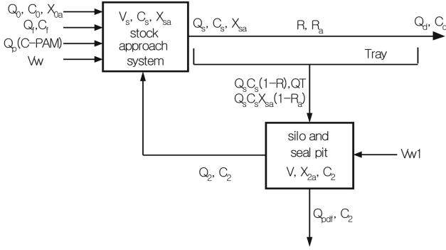
Fig. 1. Schematic of wet-end section.
